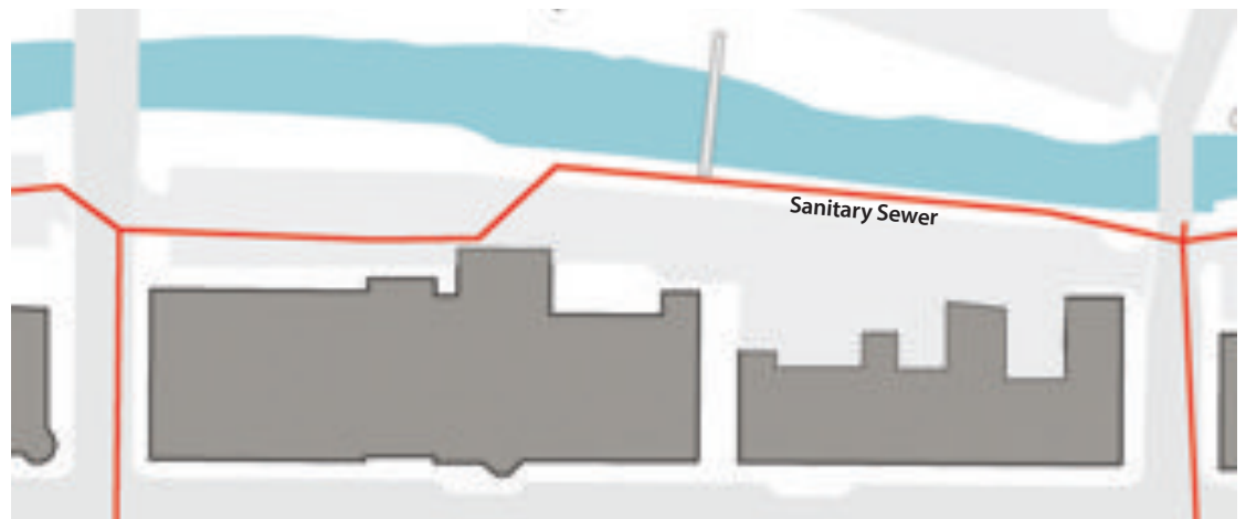
Figure 33: Sanitary sewer. A large sanitary sewer line runs parallel to the retaining wall for most of this block and should be protected. The city should take advantage of the opportunity to break down the wall where the sewer line turns south and eliminates the necessity of the wall for a stretch.
